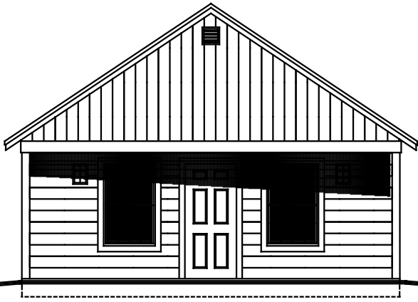
FRONT ELEVATION
