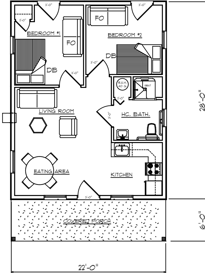
FLOOR PLAN
